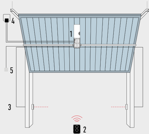
Non-projecting up-and-over door
